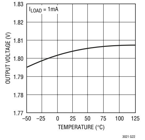
Output Voltage
